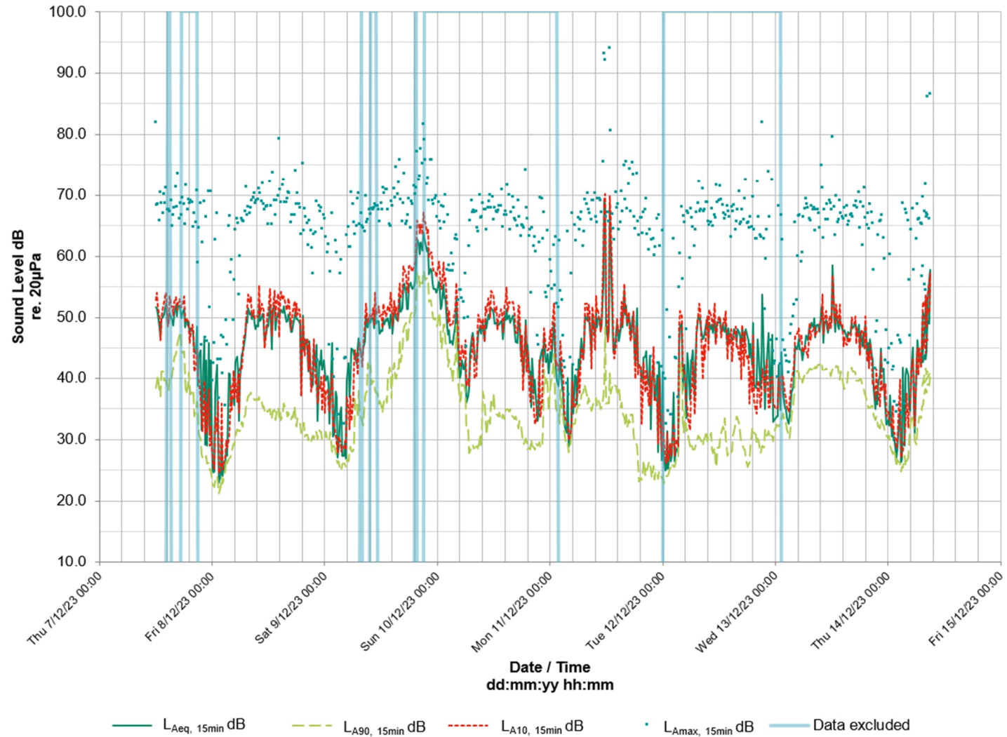
Plate 4-3: ML3 Time-History Graph
