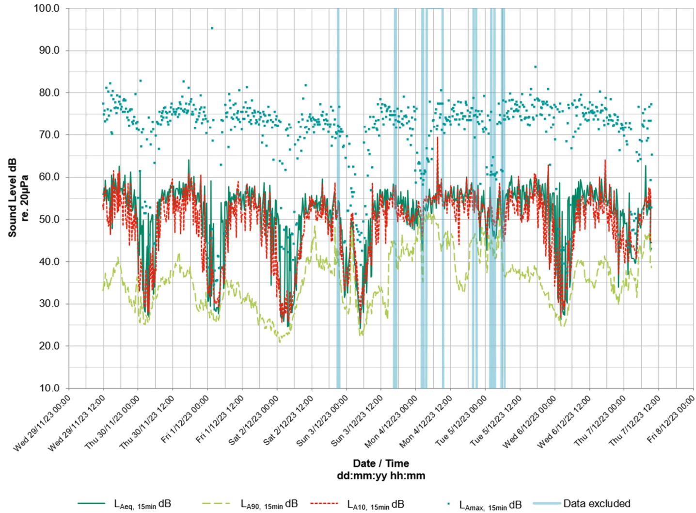
Plate 4-8: ML9 Time-History Graph
