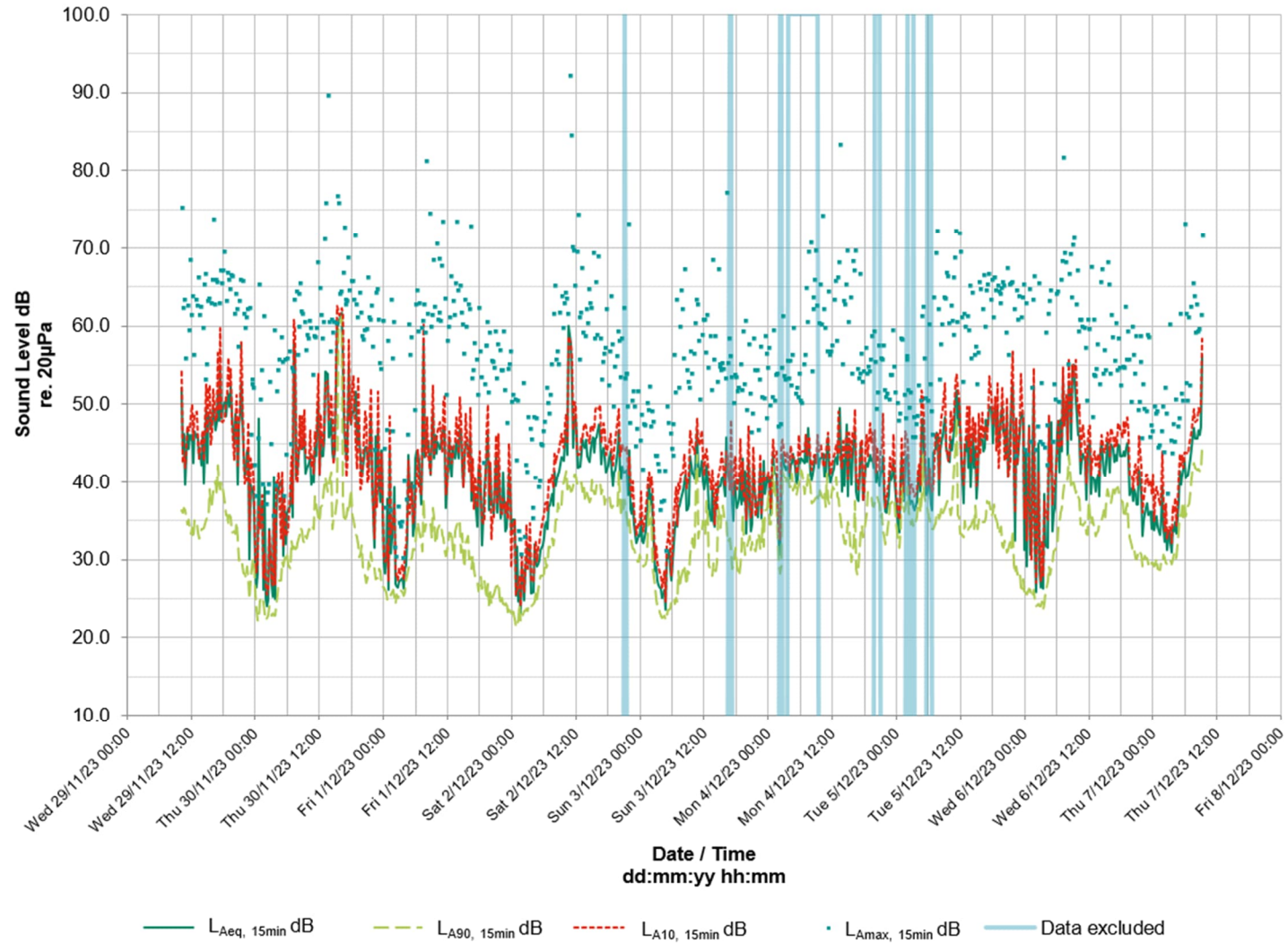
Plate 4-7: ML8 Time-History Graph
