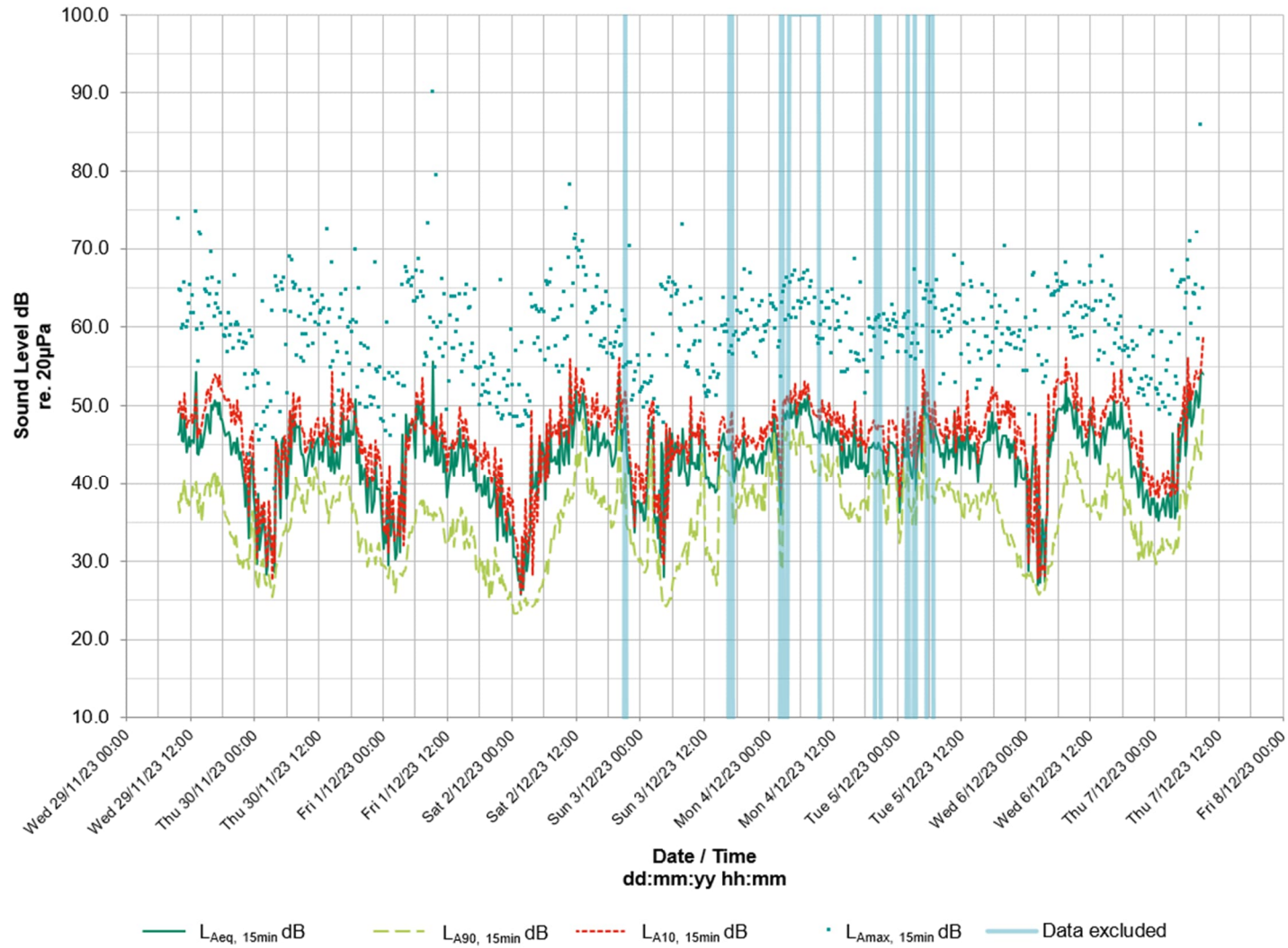
Plate 4-6: ML7 Time-History Graph
