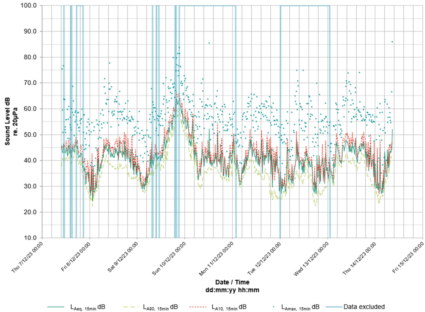
Plate 4-2: ML2 Time-History Graph
