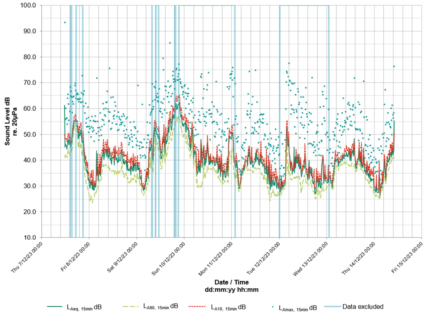
Plate 4-5: ML6 Time-History Graph
