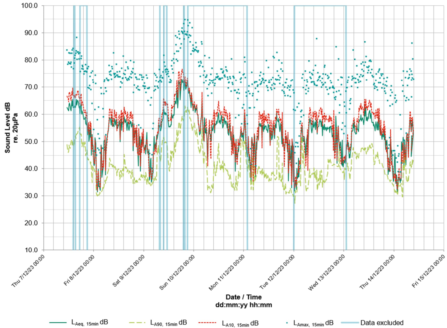
Plate 4-4: ML5 Time-History Graph
